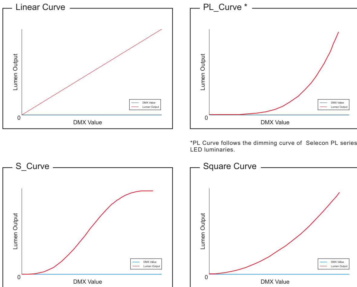
Figure 14: SL NITRO 510C LED STROBE Luminaire Dimmer Curves
