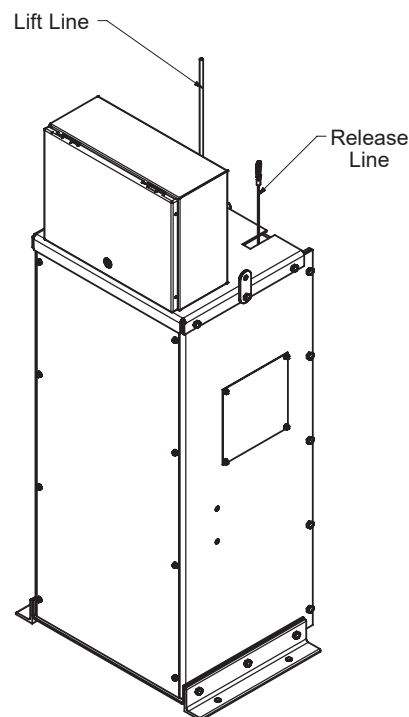
Motorized Fire Curtain Hoist
