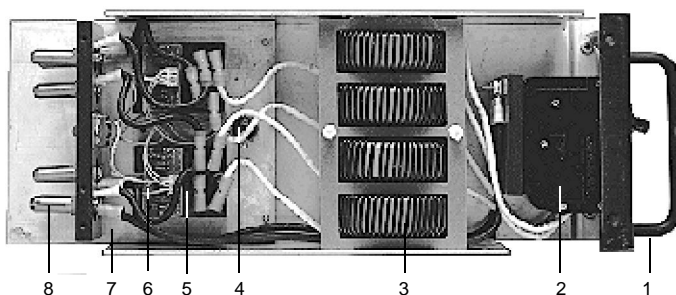
2x2 Pro Module side view with coverplate removed
