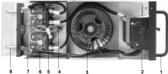
2x6 Module side view with coverplate removed
