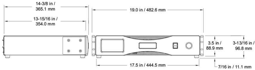
Figure 2: Neo X Server Dimensioned drawings
