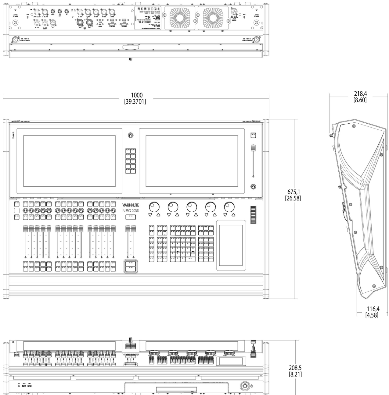
Figure 2: Neo X15 Dimensioned drawings
