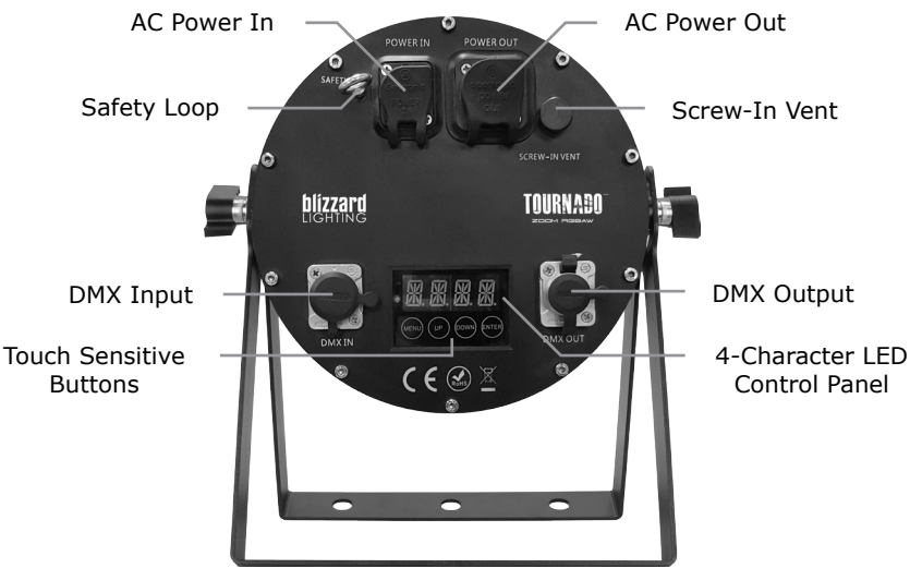
Figure 2: The Rear Connections
